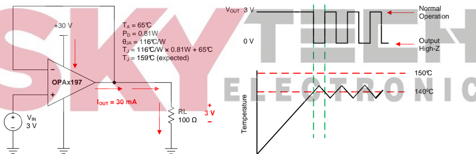
Figure 46. Thermal Protection
