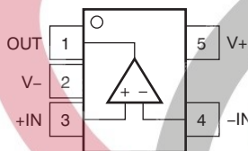
DBV Package: OPA197 5-Pin SOT Top View
